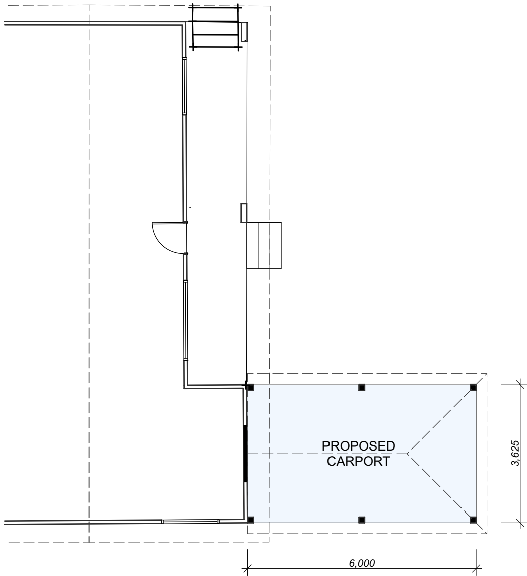
CARPORT FLOOR PLAN 1:100
