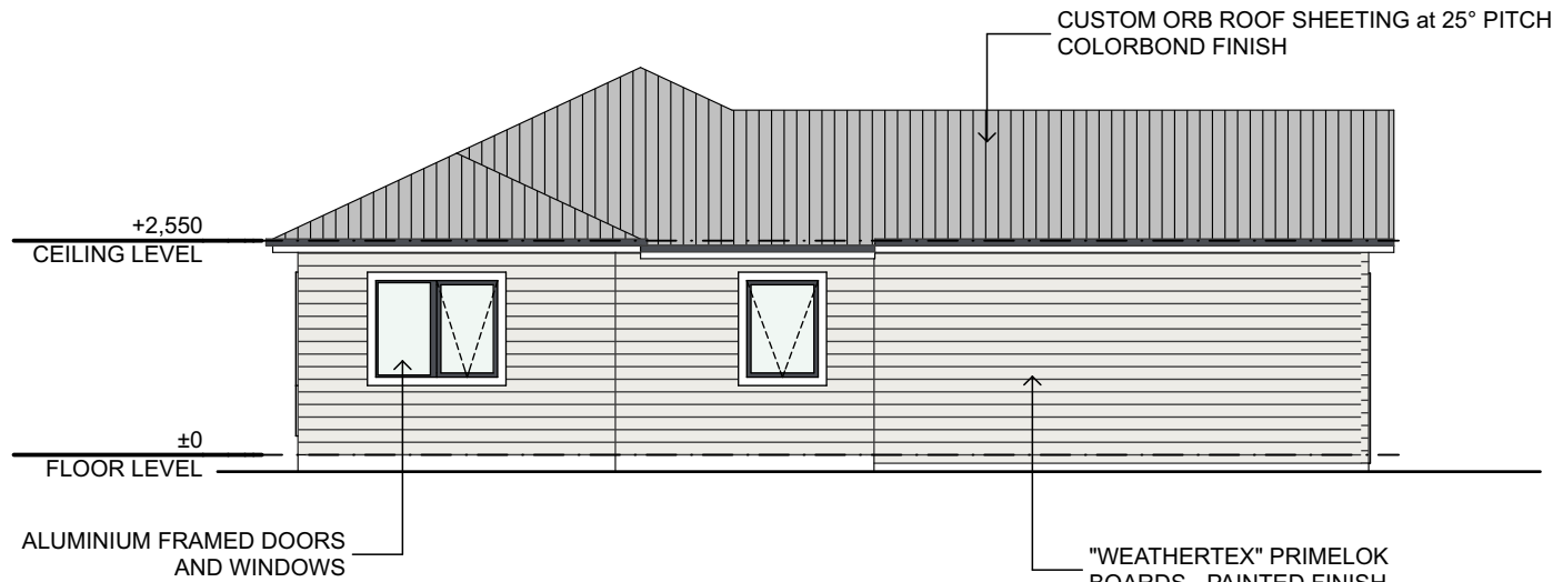
EAST ELEVATION - DWELLING 1 1:100
