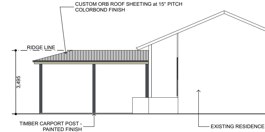
NORTH ELEVATION - CARPORT 1:100
