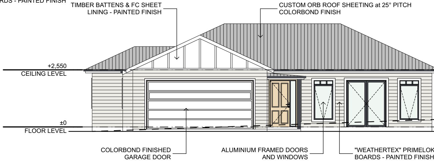
NORTH ELEVATION - DWELLING 1 1:100
