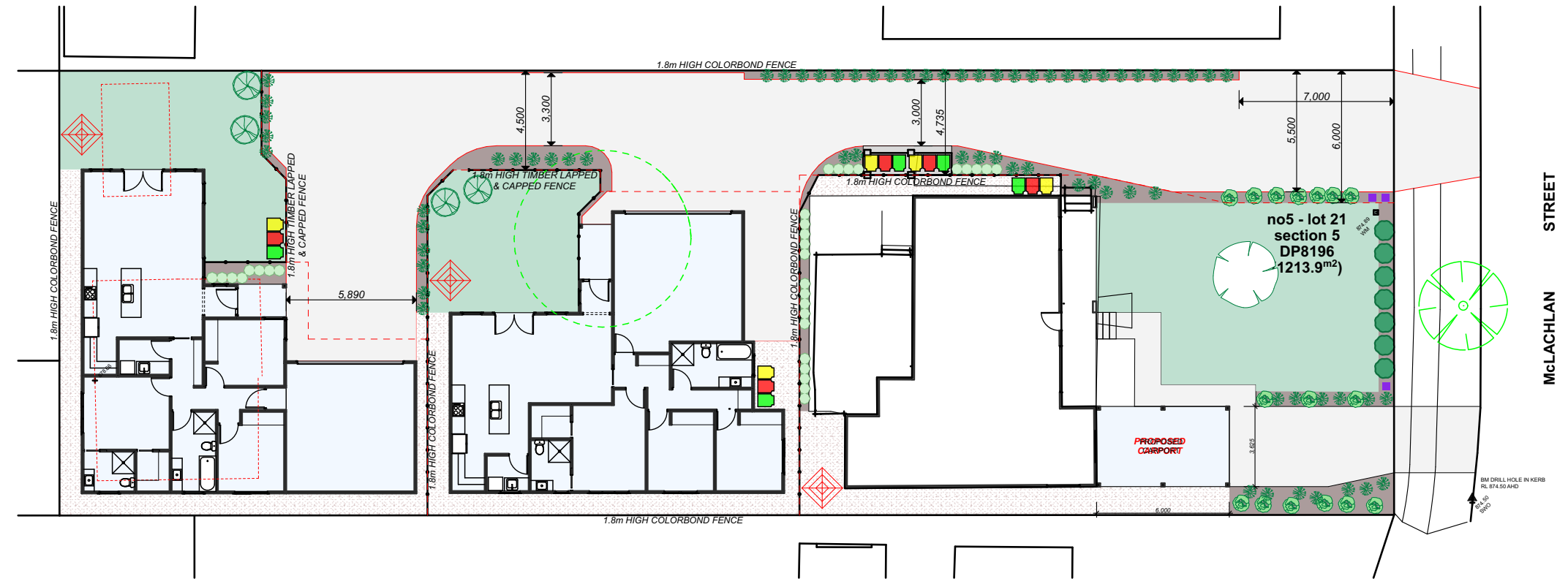
LANDSCAPING PLAN 1:250
