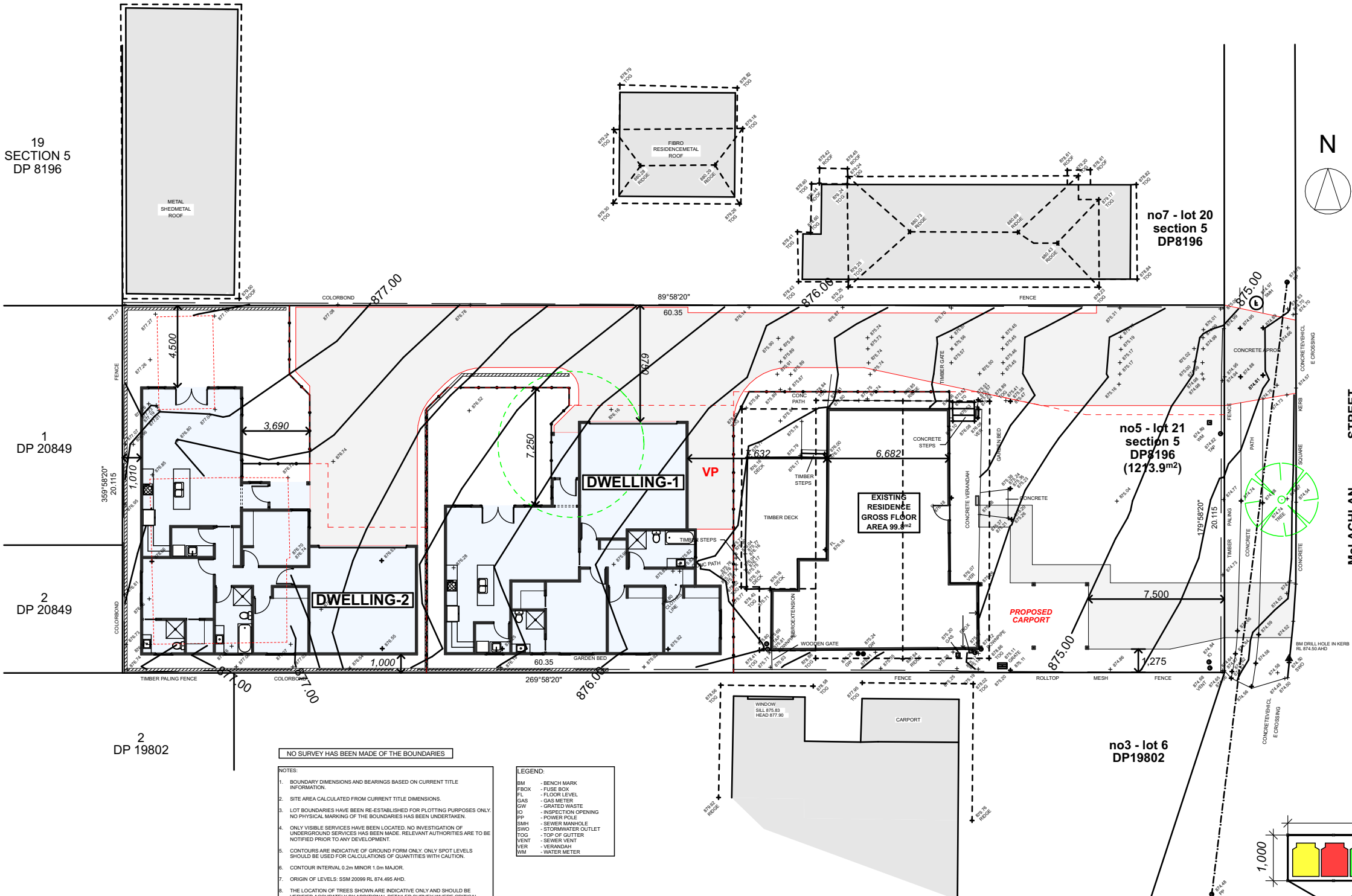
PROPOSED SITE PLAN 1:250
