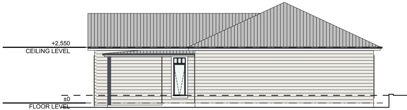
WEST ELEVATION - DWELLING 1 1:100
