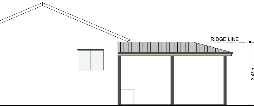
SOUTH ELEVATION - CARPORT 1:100
