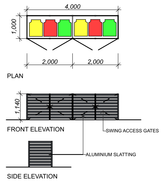
GARBAGE ENCLOSURE 1:100
